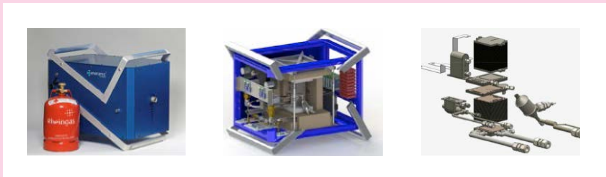
Figure 18: SOFC 100W system from Eneramic, showing the whole system, a view into the system and the stack and fuel processing components.
