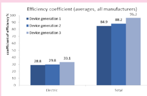
Figure 16: Efficiency coefficient (CE test standard) for CHP FC generation 1, 2 and 3 under the Callux project
