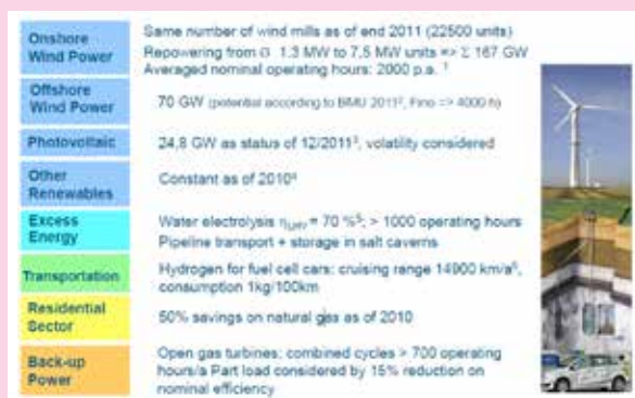
Figure 25: Scenario of the energy system for Germany in view of a 55% CO 2 reduction, developed by the Institute of Electrochemical Process Engineering (IEK-3) (Source: Forschungszentrum Jülich)
